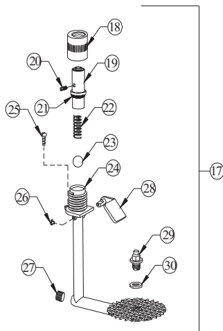
WATER SUPPLY CONNECTION
