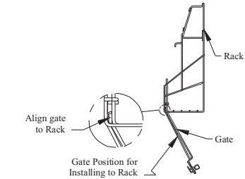
GATE INSTALLATION DETAIL
