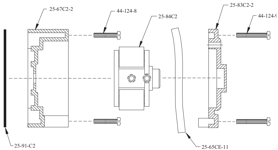
C2 PUMP ASSEMBLY
