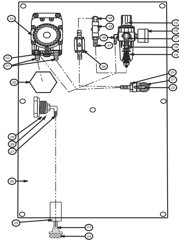
INSIDE VIEW - CONTROL PANEL
