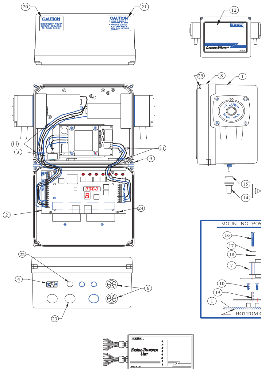
(27) SIGNAL TRANSFER UNIT (STU)
